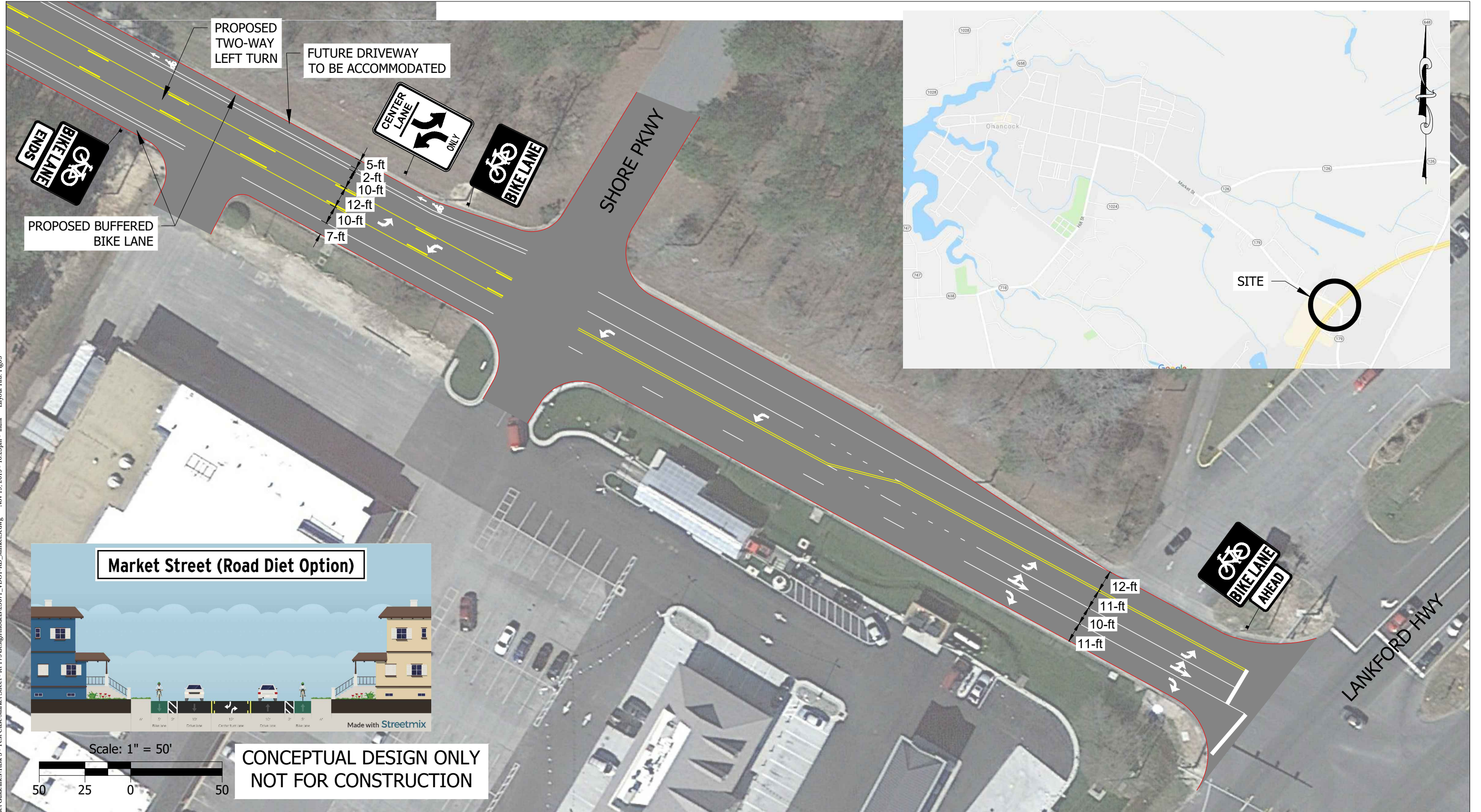
Market Street Road Diet Concept Lakeside Avenue Transition Accomack County, Virginia
