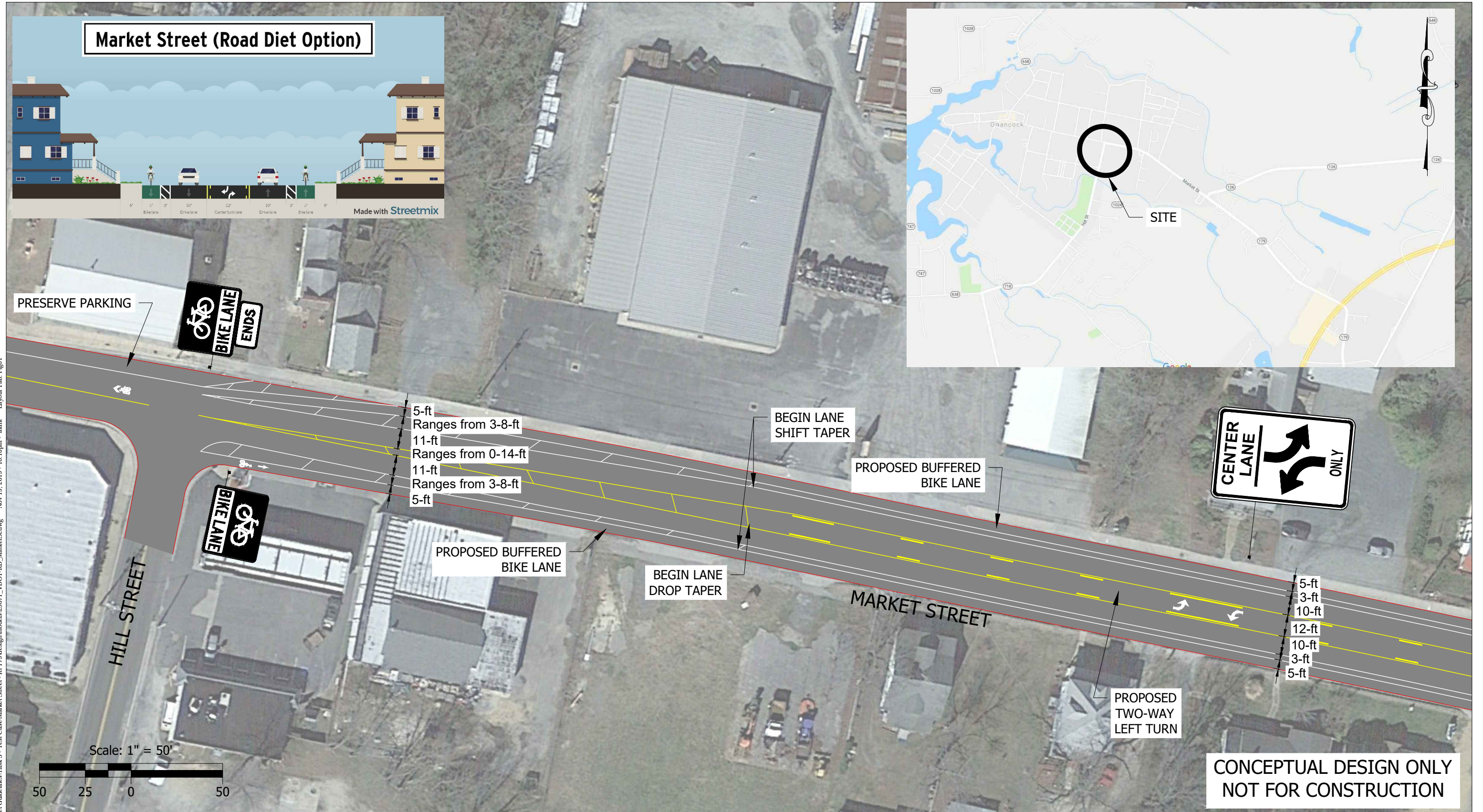
Market Street Road Diet Concept Hill Street Transition Accomack County, Virginia
