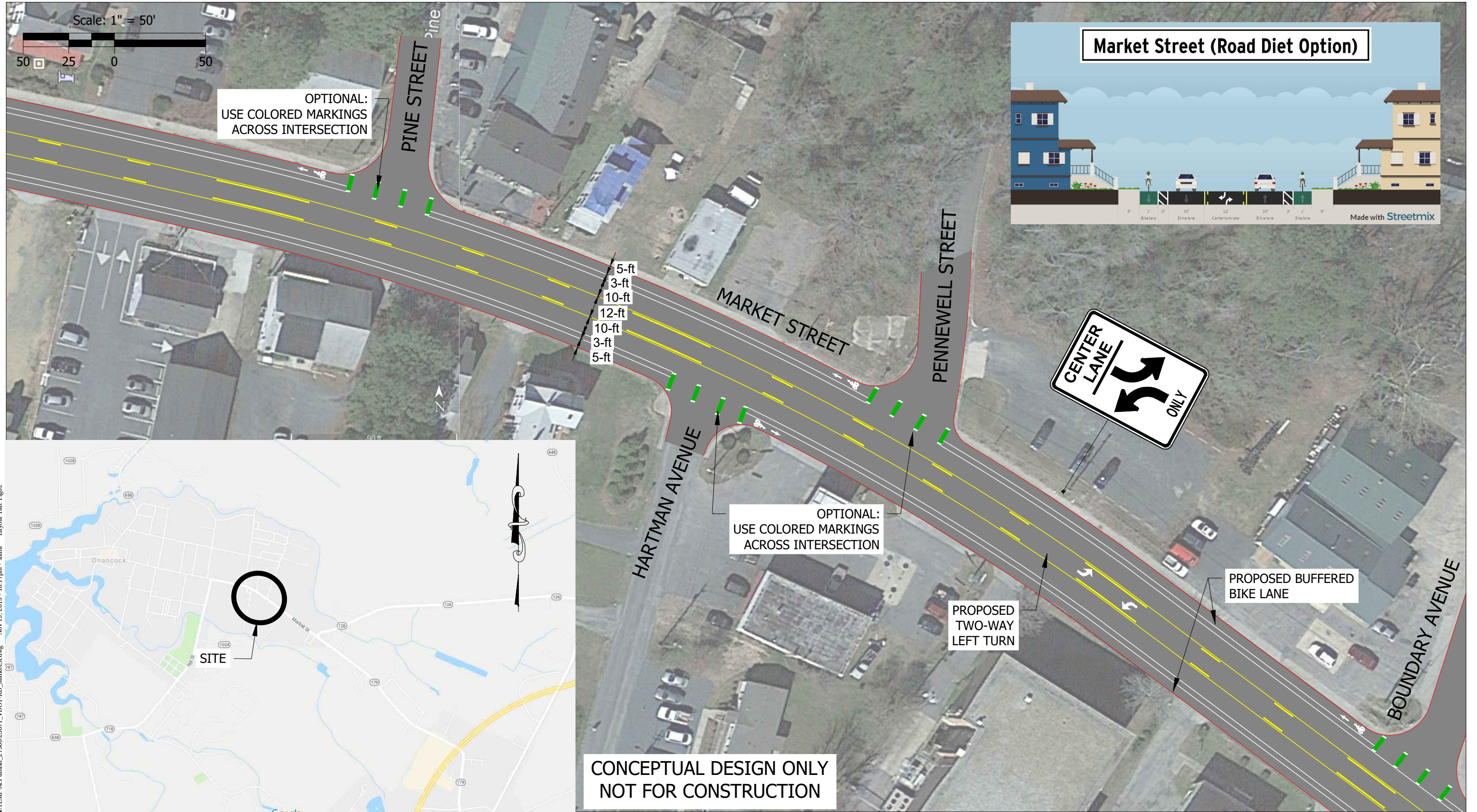
Market Street Road Diet Concept Hall Street Transition Accomack County, Virginia
